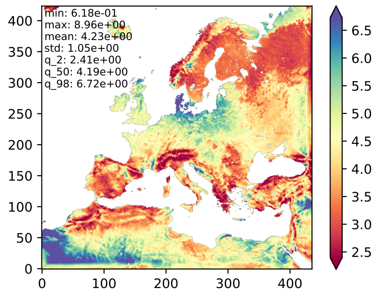
WIND mean
