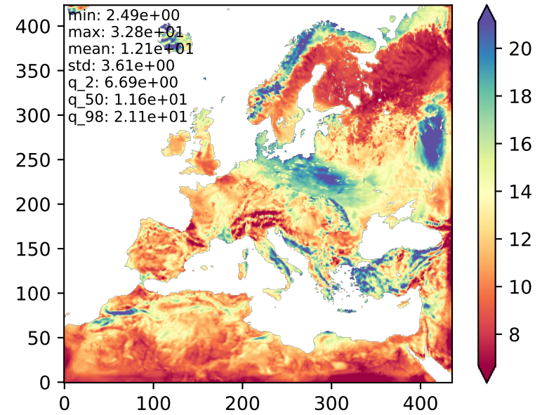
WIND mean - distribution
