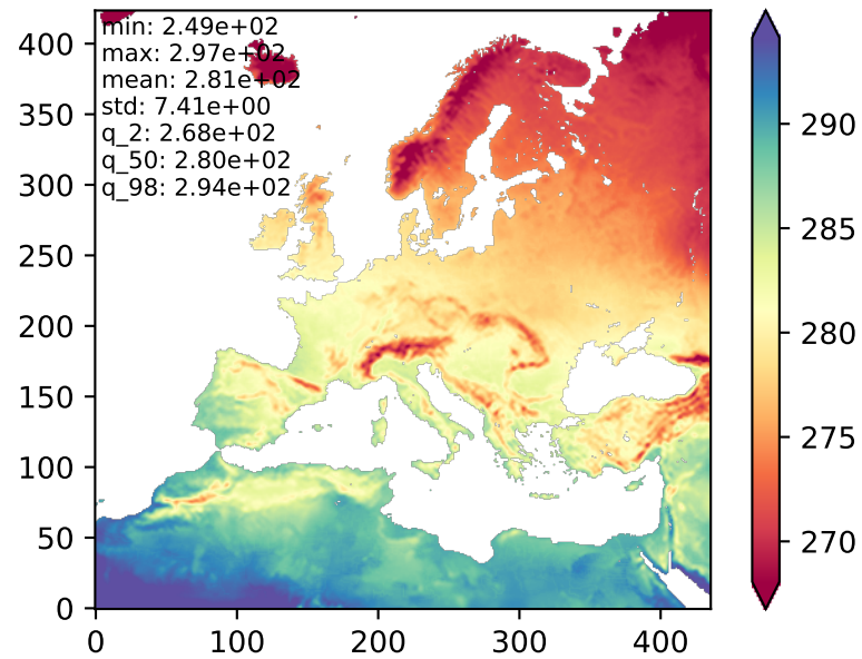
THBOT mean
