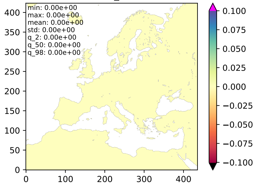
RUNOFF_T mean - distribution
