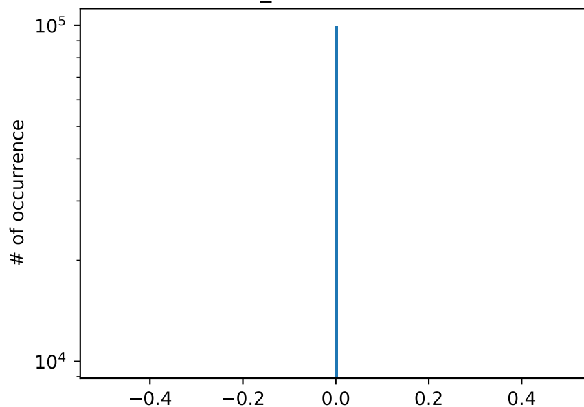
RUNOFF_T mean - distribution
