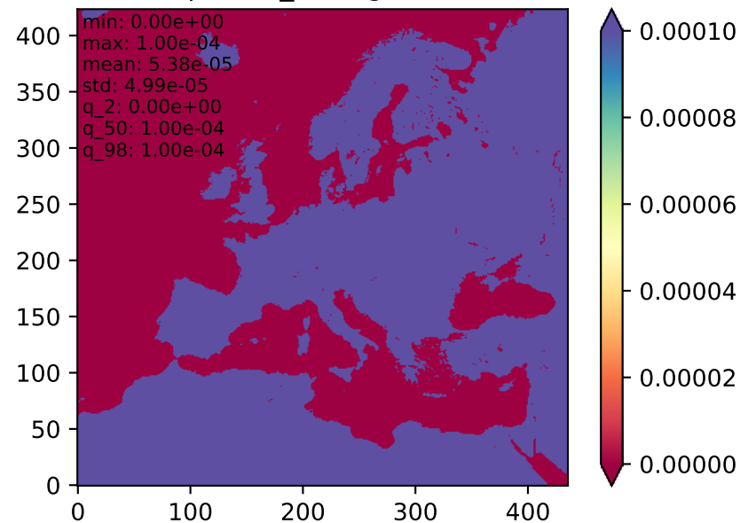
specific_storage mean - distribution
