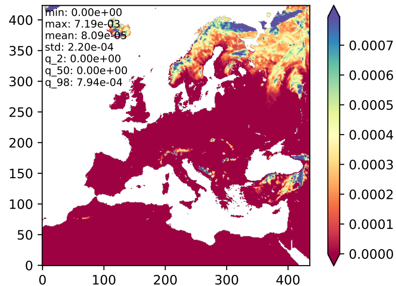
SNOW mean - distribution
