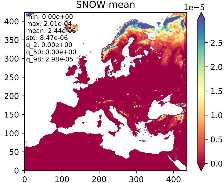
SNOW mean
