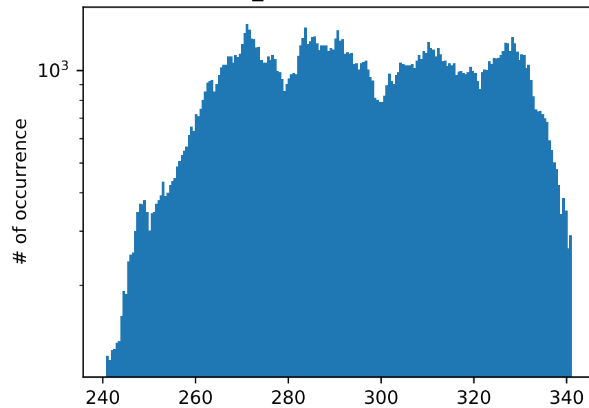
ALWD_S mean - distribution
