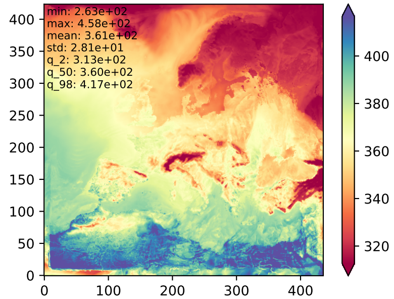
ALWD_S mean - distribution
